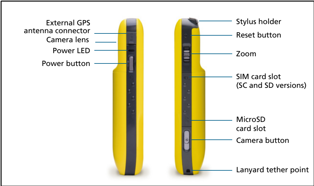
Figure 2.3 Juno series handheld – left and right views
